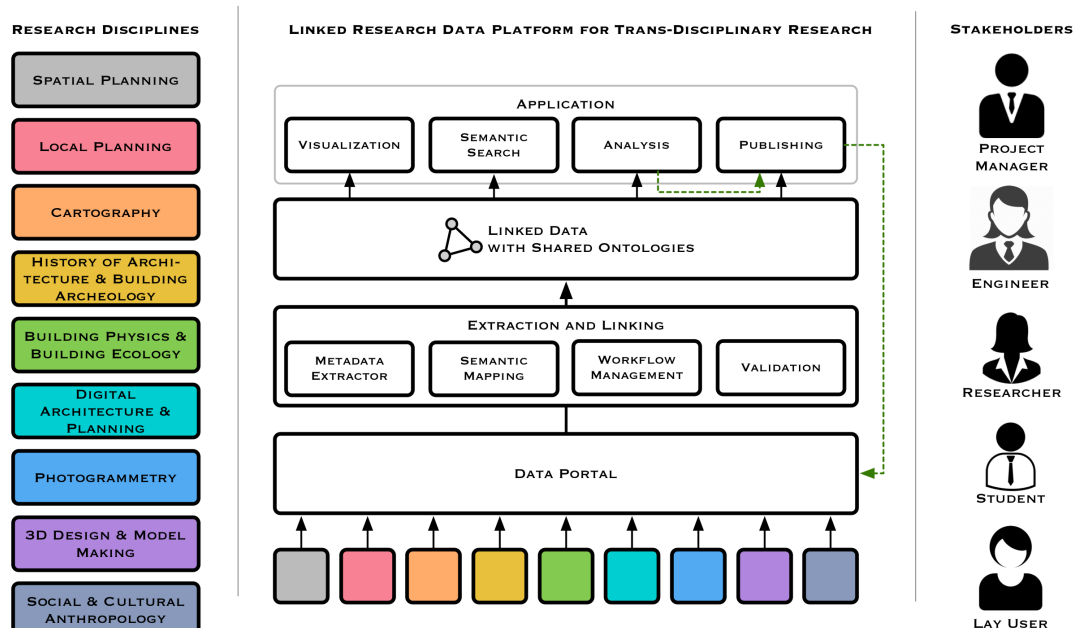
Figure 1: Architecture Overview
